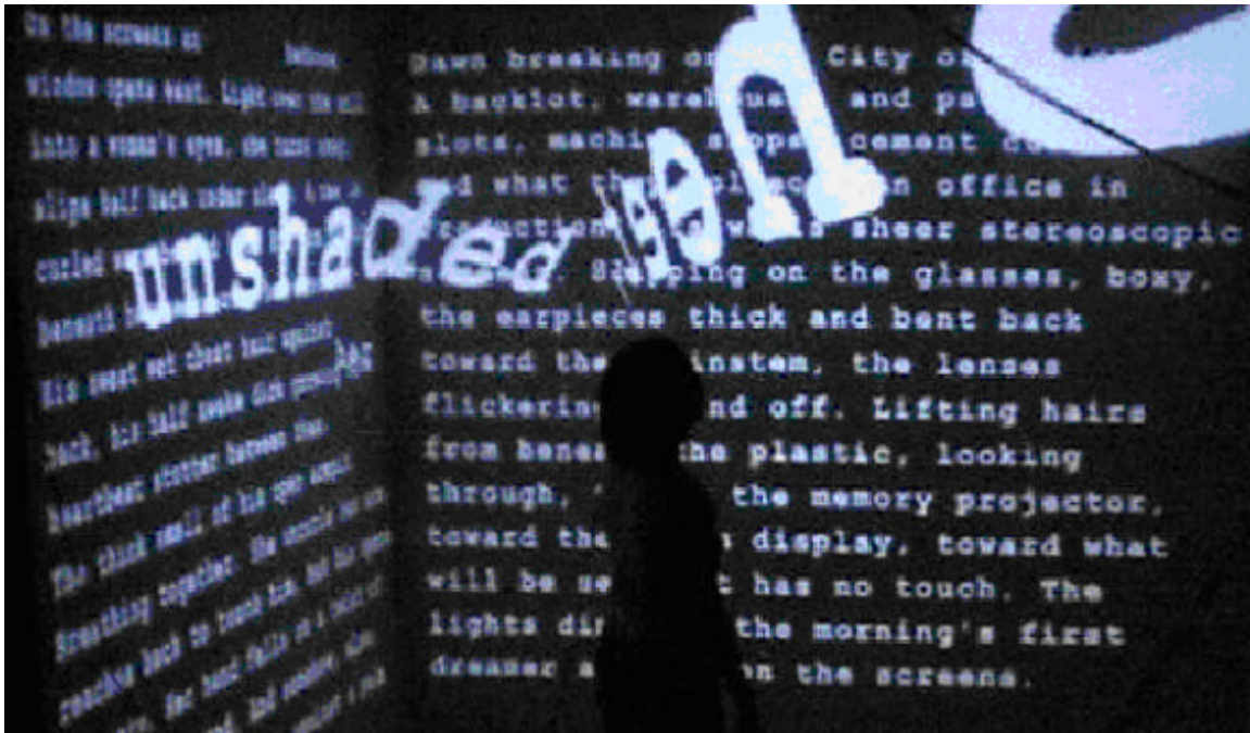
Figure 1 : Screen 7
