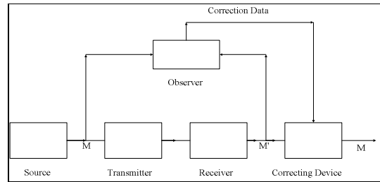
Fig 2. Schematic diagram of a correction system [14]
